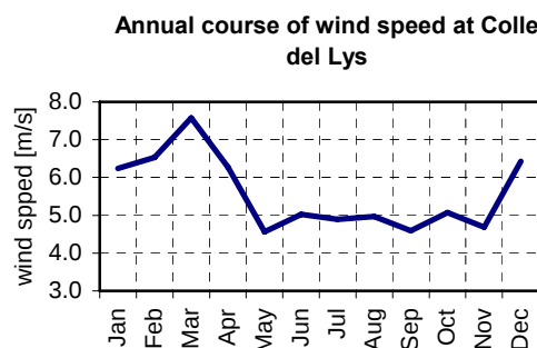
Fig. 3.1.5.2: Annual course of mean wind speed measured at Colle del Lys.
