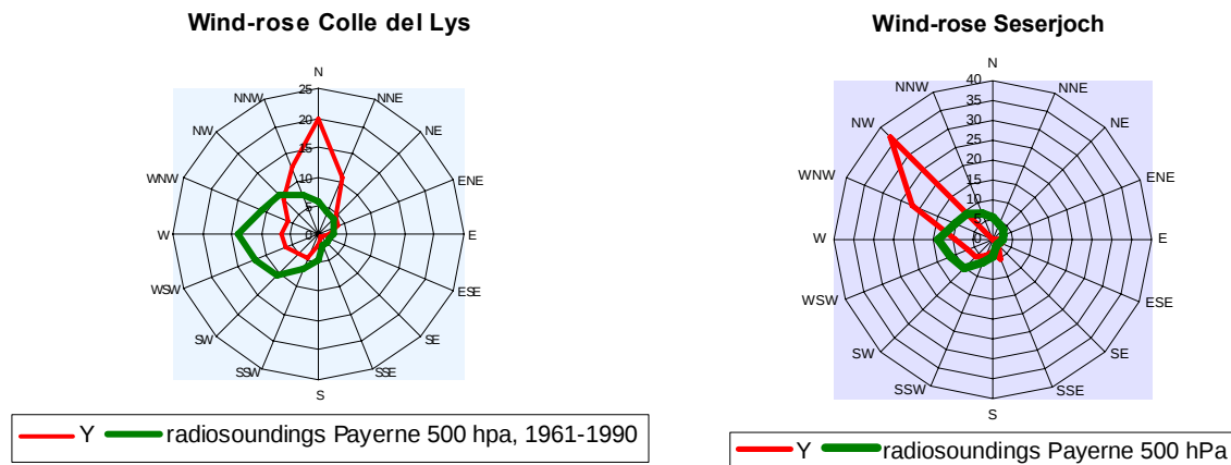
Fig. 3.1.5.1. Mean wind direction distribution for Seserjoch and Colle del Lys (Monte rosa) compared to radio sounding data of Payerne
