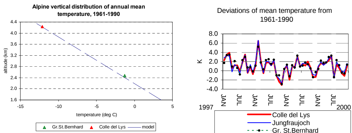
Fig. 3.1.2.1. Validation of the vertical Alpine temperature model by on-site measurements of Colle del Lys and climate data of Jungfraujoch and Großer St.Bernhard
