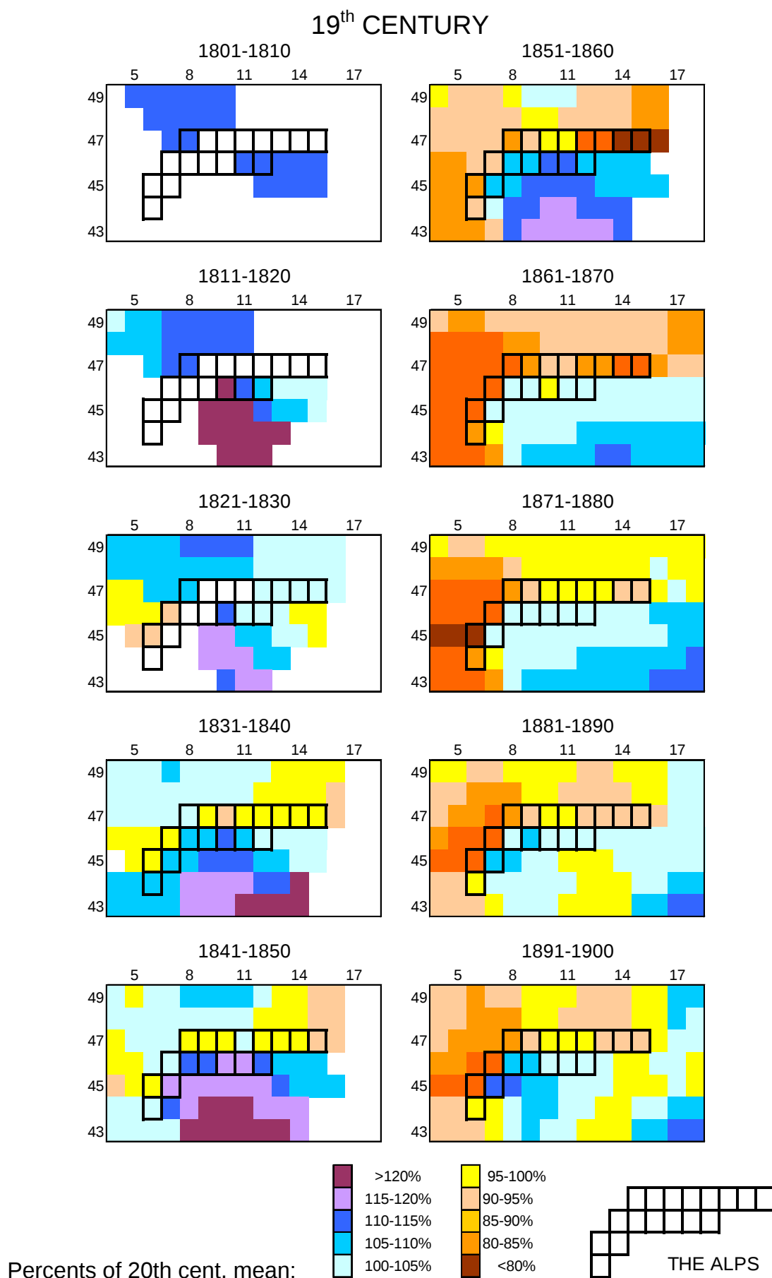
Fig. 3.2.14. Spatial patterns of decadal mean precipitation variability in the greater alpine region in the 19 th century.
